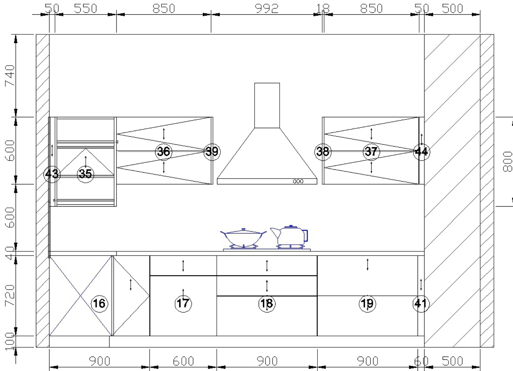
D View elevation drawing
