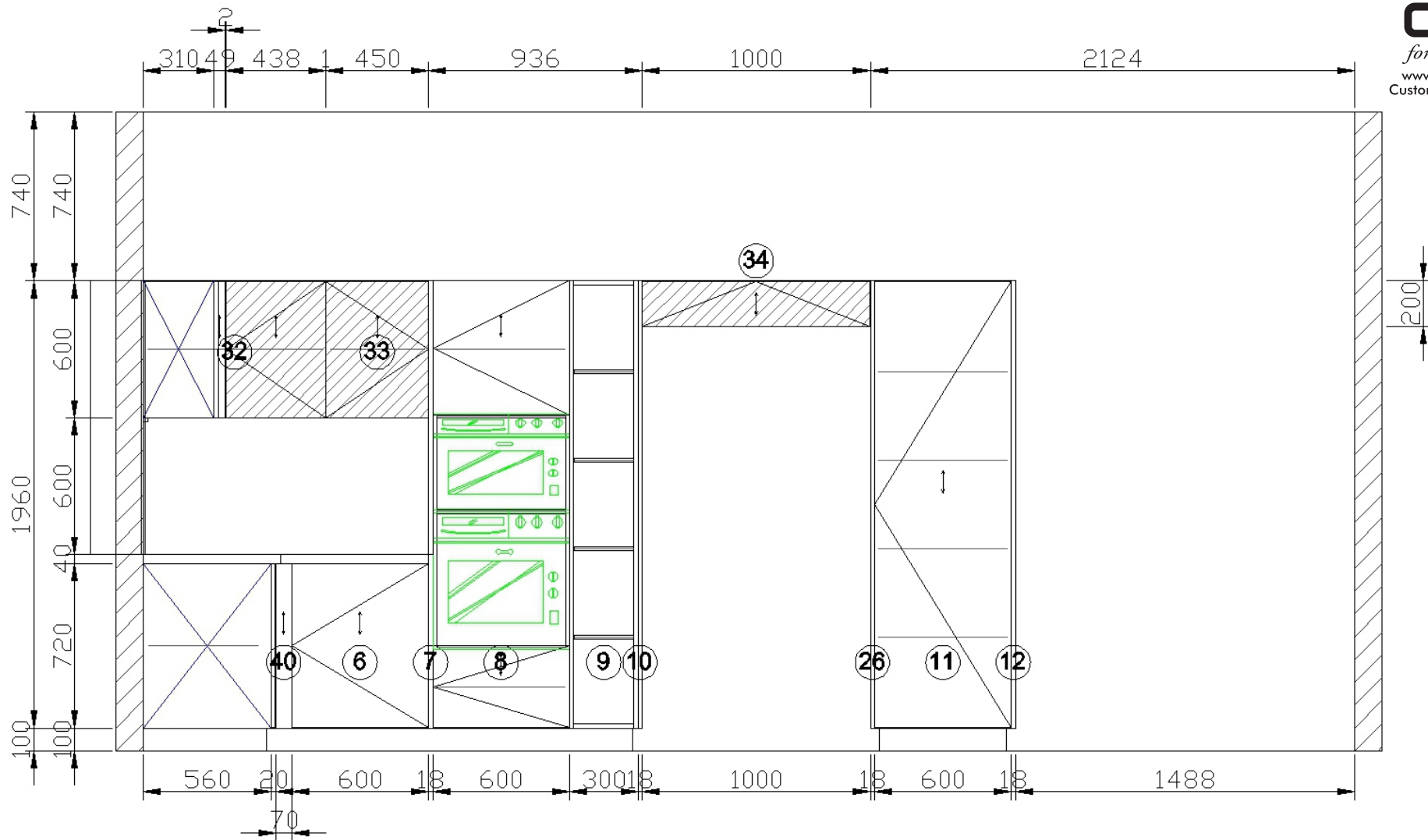
B View elevation drawing
