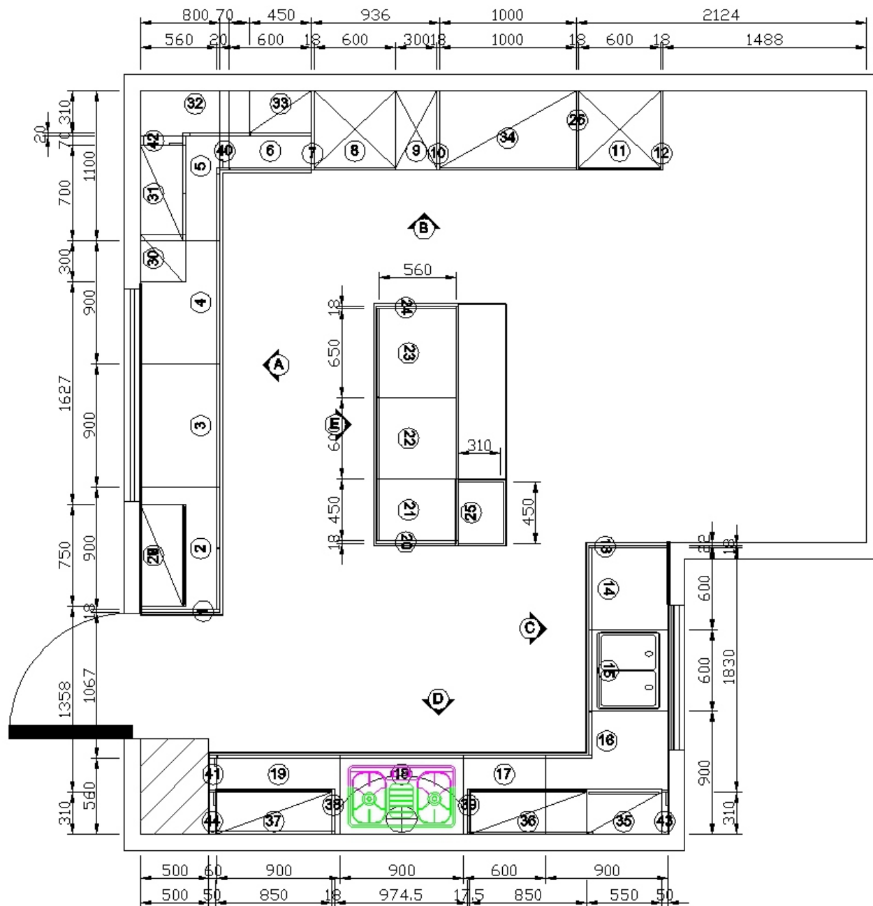
Plan drawing
